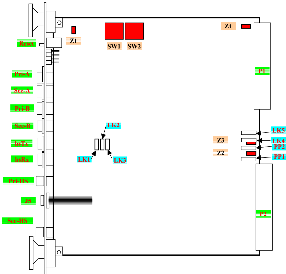
Figure 1-3 Location of Address Switches and Linkers diagram
